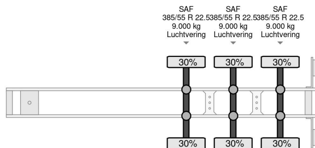
Van Hool 3 AXLE MULTICHASSIS - EXTENDABLE
