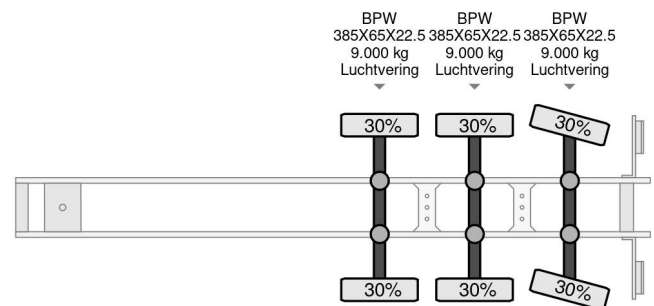
VAN ECK 3 AXEL CARRIER VECTOR 1850 D/E
