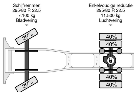
DAF XF 105.460 SC 4X2 EURO 5 MANUAL
