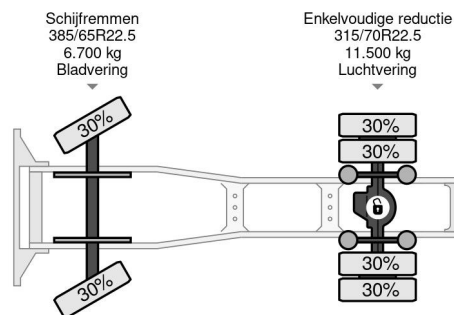
Volvo FH 12.460 4X2 SPOILERS EURO 3 MANUAL
