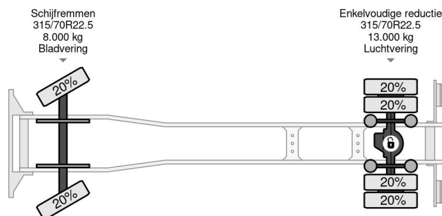
DAF CF 290 4X2 - EURO 6 + HEATING SYSTEM + BÄR CA...
