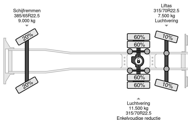
Scania P320 6X2 - EURO 6 + HIAB XS 144 HIPRO + REMO...
