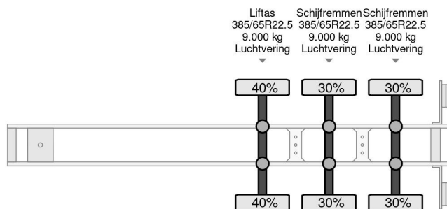
Schmitz Cargobull SGF*3 LIFTING AXLE
