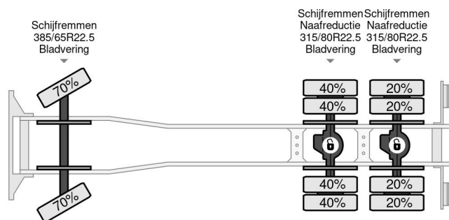
Iveco Trakker 500 6X4 EURO 6 KIPPER + PALFINGER PK18...
