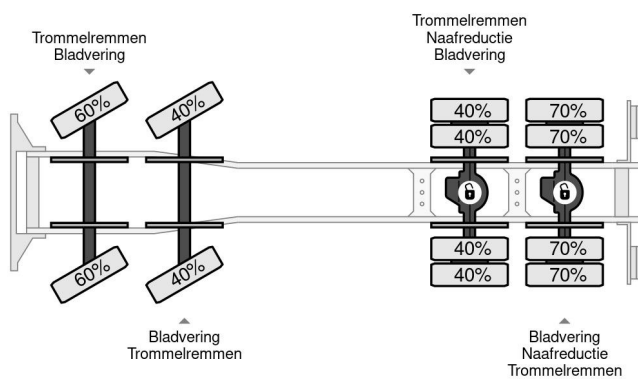
Scania P410 8X4 KH KIPPER FULL STEEL EURO 6D
