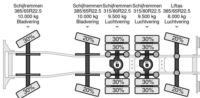
Scania G450 10X4 3 UNITS VAKO KIPPER EURO 6
