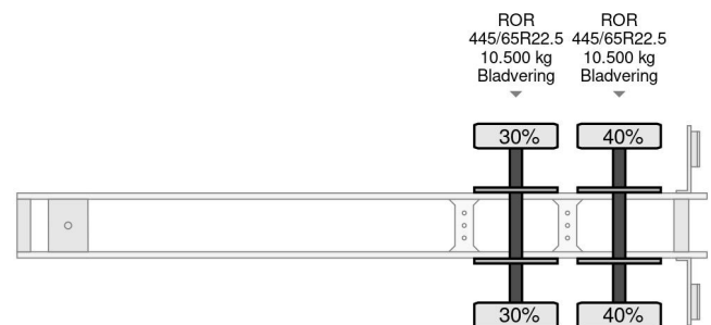
CIF 2 AXLE - STEEL SUSPENSION - TIPPER
