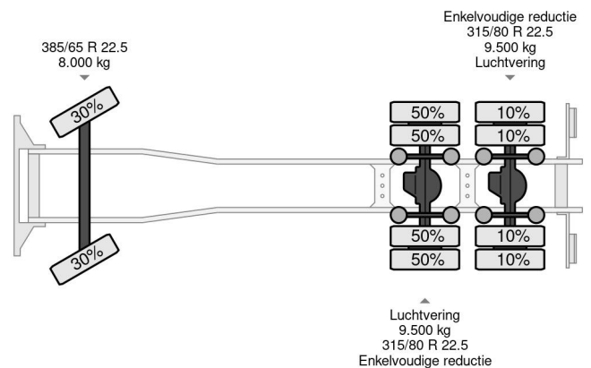
Scania R560 V8 6X4 Euro 5 CableLift
