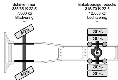
DAF XF 105.460 4X2 SSC EURO 5 RETARDER + MANUAL ...
