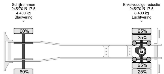
MAN TGL 12.220 4X2 EURO 5 - 12 TONS + DHOLLANDIA
