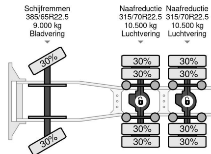
DAF XF 105.460 6X4 EURO 5 + HMF 4220 K6 + REMOTE ...
