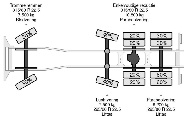
Scania R113-380 8X2/4L - HOOKLIFT - MANUAL GEARBOX
