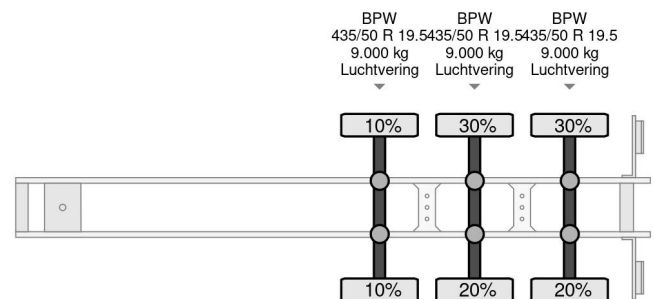
LAG 3 AXLE MEGA 1360x249x304
