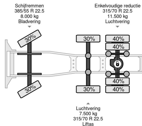
MAN TGX 26.460 6X2-2 EURO 6 LIFT AXLE
