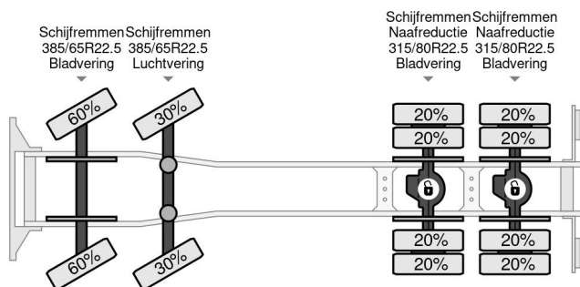
Scania R730 V8 8X4 EURO 6 BIG AXLES
