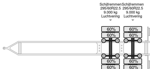
Fliegl TPS 180 - 2 AXLE BPW + TRS COOLING
