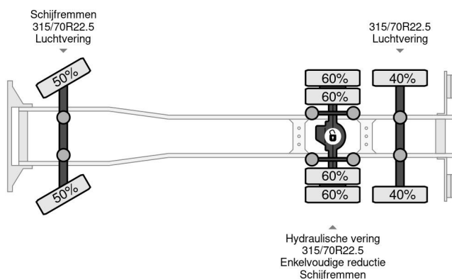
Scania P280 6X2 - EURO 6 + CNG + JOAB BINLIFT L77
