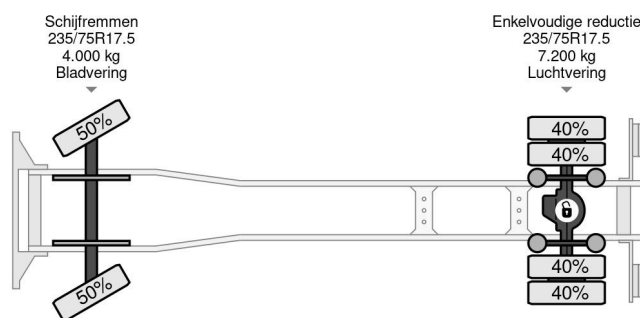
Mercedes-Benz Atego 1016 4X2 - EURO 6 + DHOLLANDIA LIFT
