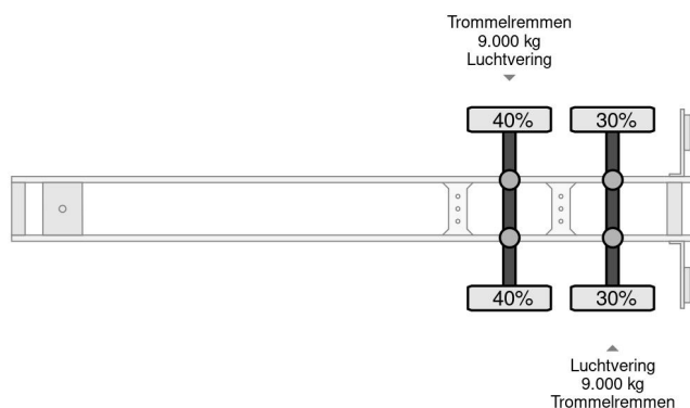
SYSTEM TRAILERS PRSH18 - 2 AXLE BPW
