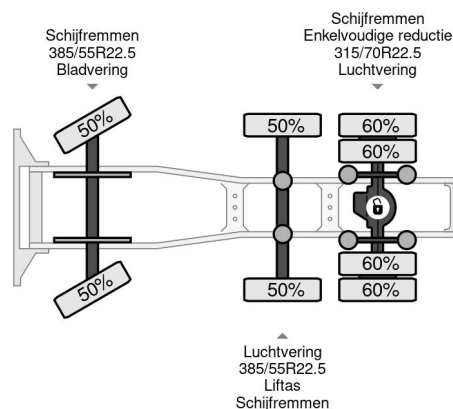
MAN TGX 26.500 6X2 EURO 6 ALCOA SPOILERS 2020
