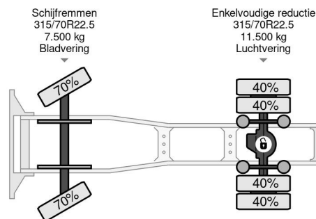
MAN TGX 18.470 4X2 DOUBLE TANK DUTCH TRUCK TÜV ...
