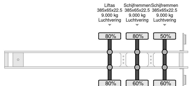
UNITRANS WITH MEATRAILS AND DOUBLE EVAPORATOR
