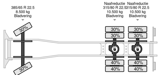
DAF CF 85.380 6X4 VACUUM CLEANER - FULL STEEL
