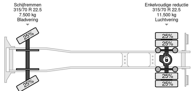
DAF CF 75.360 4X2 EURO 5 + PALFINGER PK15500
