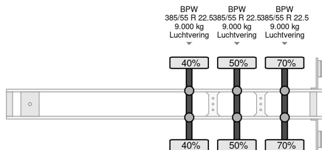
TURBO'S HOET TANKCONTAINER CHASSIS - 3.920kg
