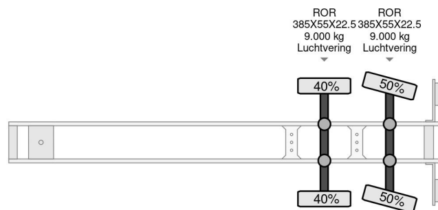
Burg LAST AXEL STEERING + LOAD LIFT
