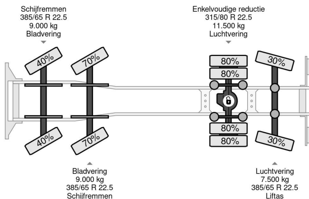
Scania R490 8X2 EURO 6 + EFFER 1750/4S + REMOTE
