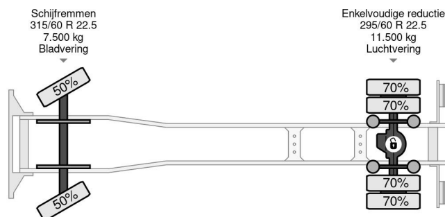
DAF CF 260 4X2 EURO 6 CARRIER SUPRA 450 NORDIC + ...
