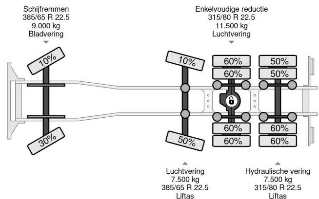
DAF XF 95.480 8X2 EURO 3 + VDL HOOKLIFT + MANUAL ...
