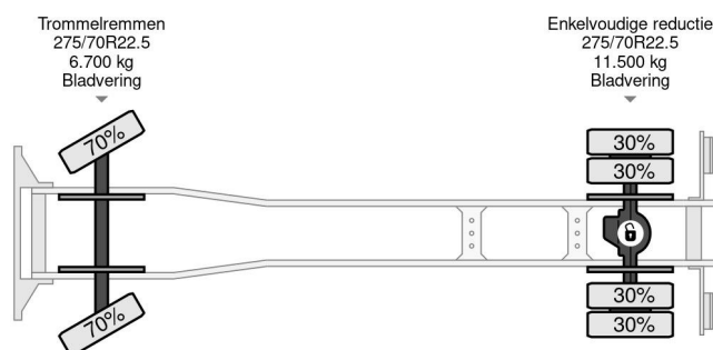
Scania P94-230 4X2 MANUAL GEAR - FULL STEEL SUSP. - ...
