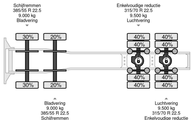
Scania R124-420 8X4 EURO 3 + EFFER 950/6S + 1 + REMOTE
