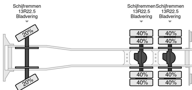
Scania P124-360 6X4 EURO 2 HIAB 200 C-5 ALL 2000
