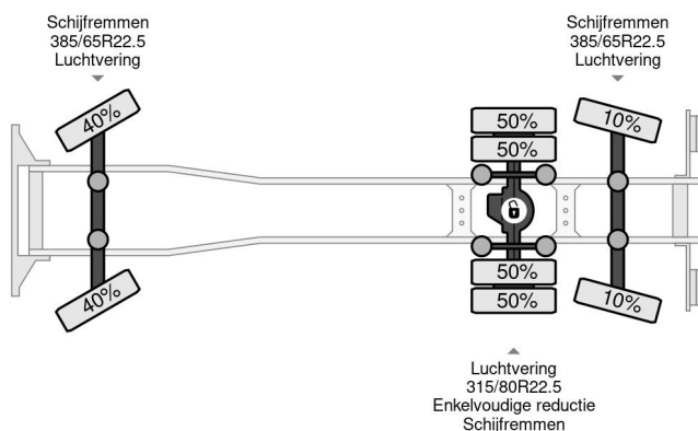
Volvo FM 500 6X2 EURO 5 HIAB 211 EP5 + REMOTE CON...
