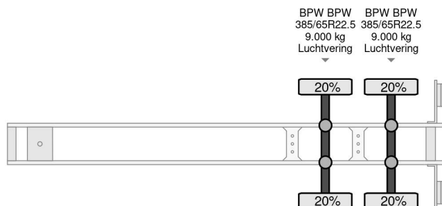
Pacton TBD230 - 2 AXLE BPW
