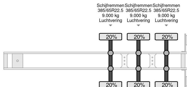
ATM OKA 17/27 - 3 AXLE
