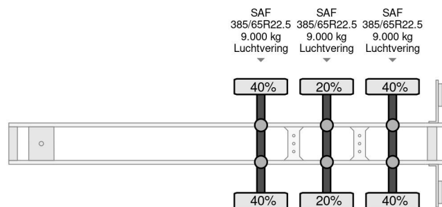
Kaiser 3 AXLE - TIPPER
