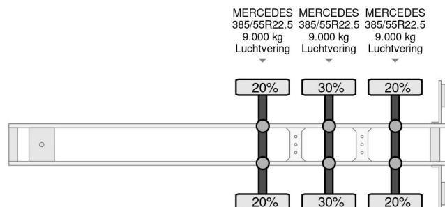
Schwarz Müller 3 AXLE + COILGOOT + SLIDING ROOF
