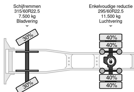
DAF CF 85.360 4X2 - EURO 5 - NL TRUCK
