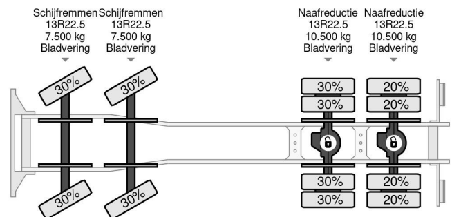
DAF CF 85.410 8X4 EURO 5 - FULL STEEL - HUB REDUCT...
