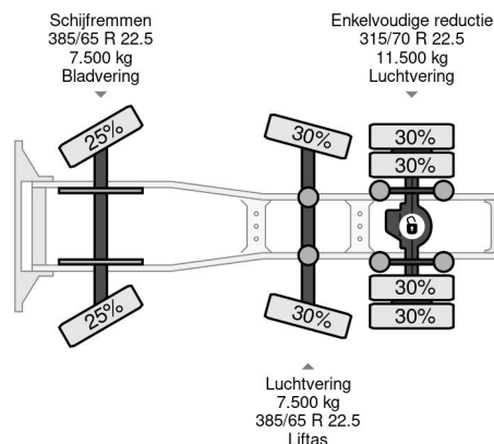
DAF XF 105.460 SSC 6X2 EURO 5 MANUAL GEARBOX
