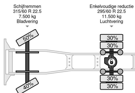
DAF CF 85.360 4X2 EURO 5 MEGA
