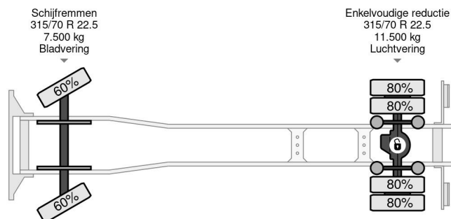
DAF CF 260 4X2 KONVEKTA COOLING + HEATING + LOAD...
