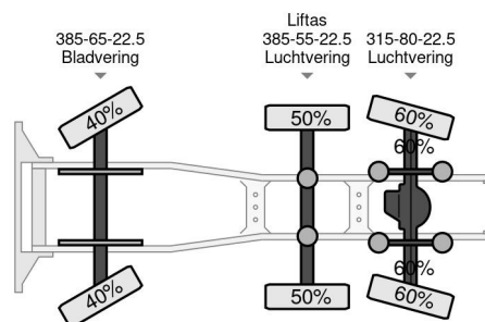
Volvo FH 500 6X2 ADR i-Shift + HYDRAULIC
