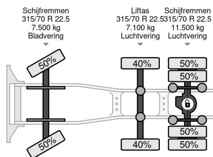
DAF XF 105.460 SSC 6X2 EURO 5
