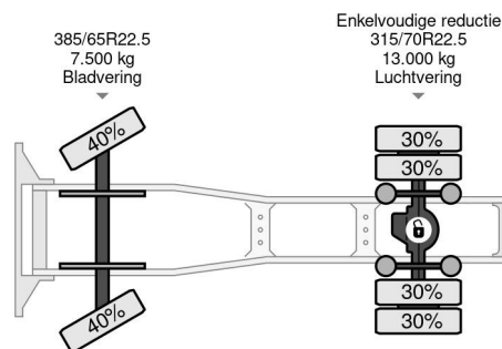
DAF XF 460 4X2 - EURO 5
