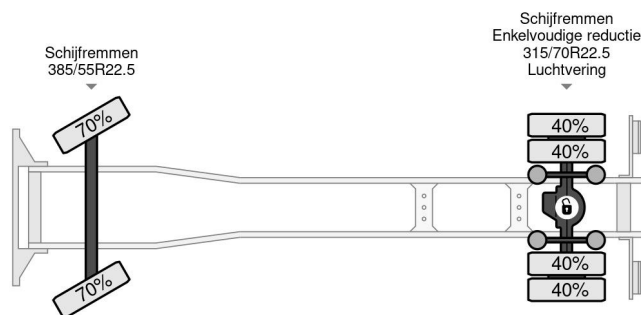
Volvo FM 330 4X2 EURO 5 JOAB SKIP LOADER
